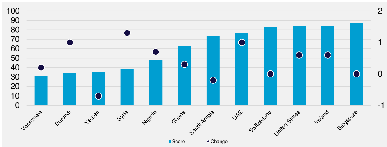
Figure 5.1: GFSI Scores
